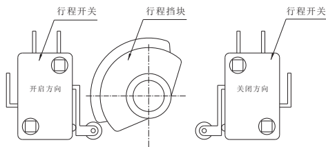
CX-20/40/60/100/200行程挡块和行程开关布局图
